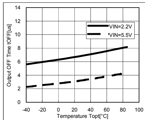
8) Output Off Time vs. Temperature
